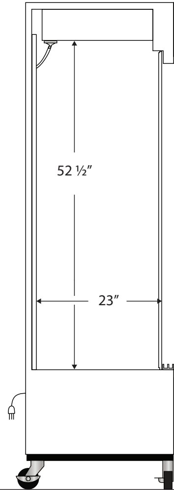
Side View
