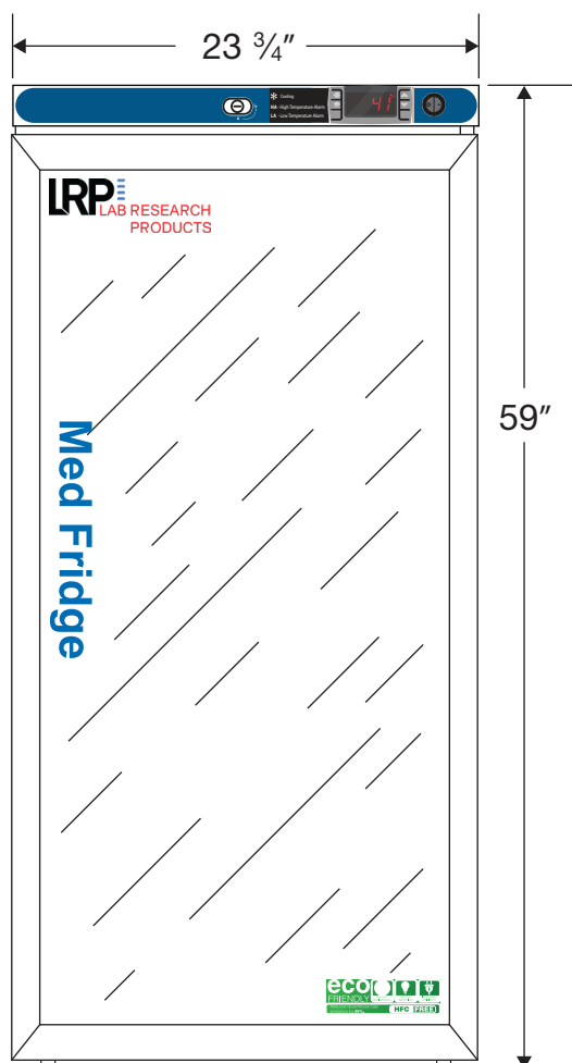
Front View
