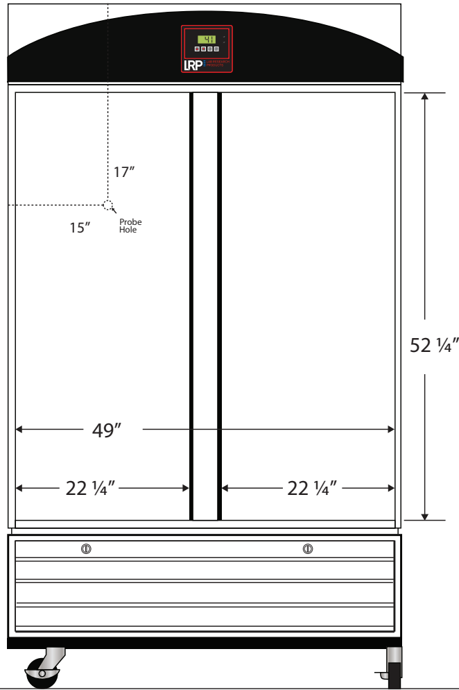
Front View
