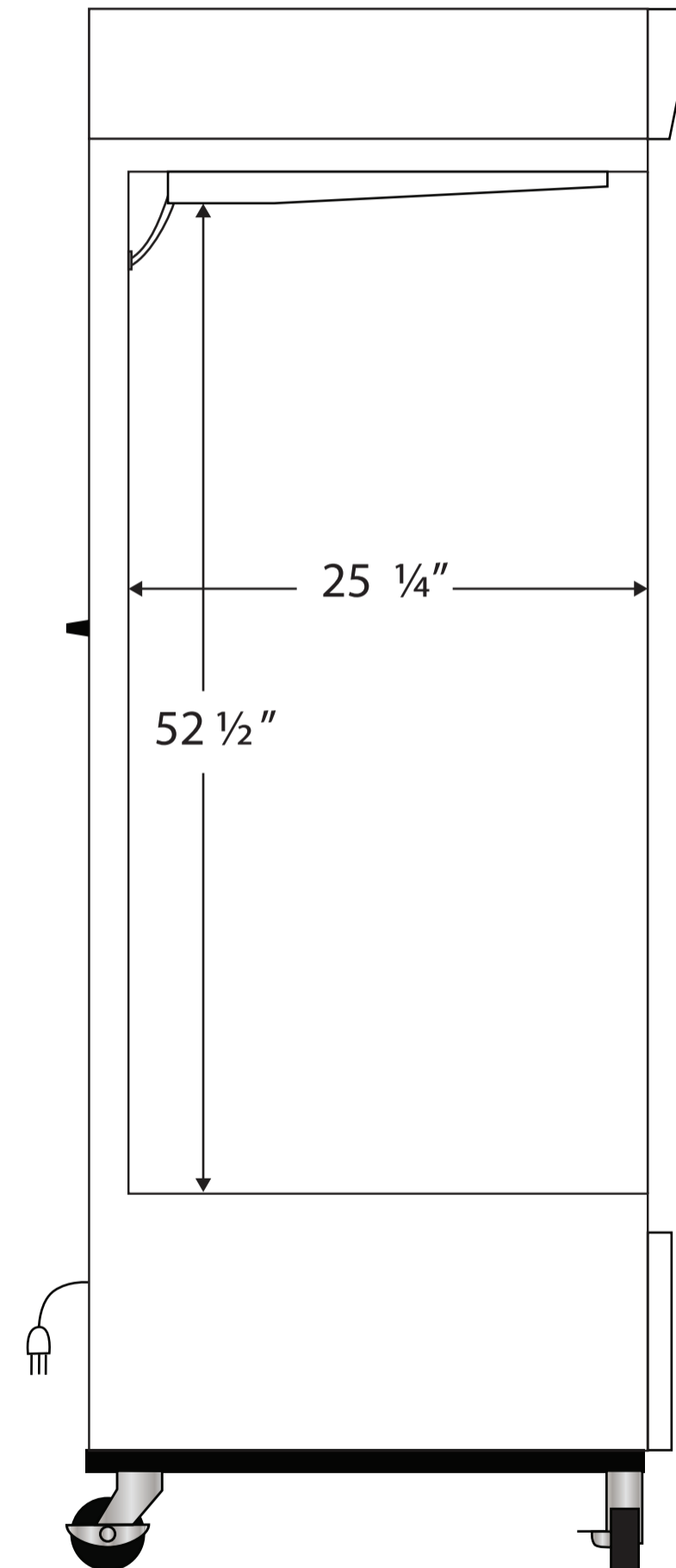
Side View
