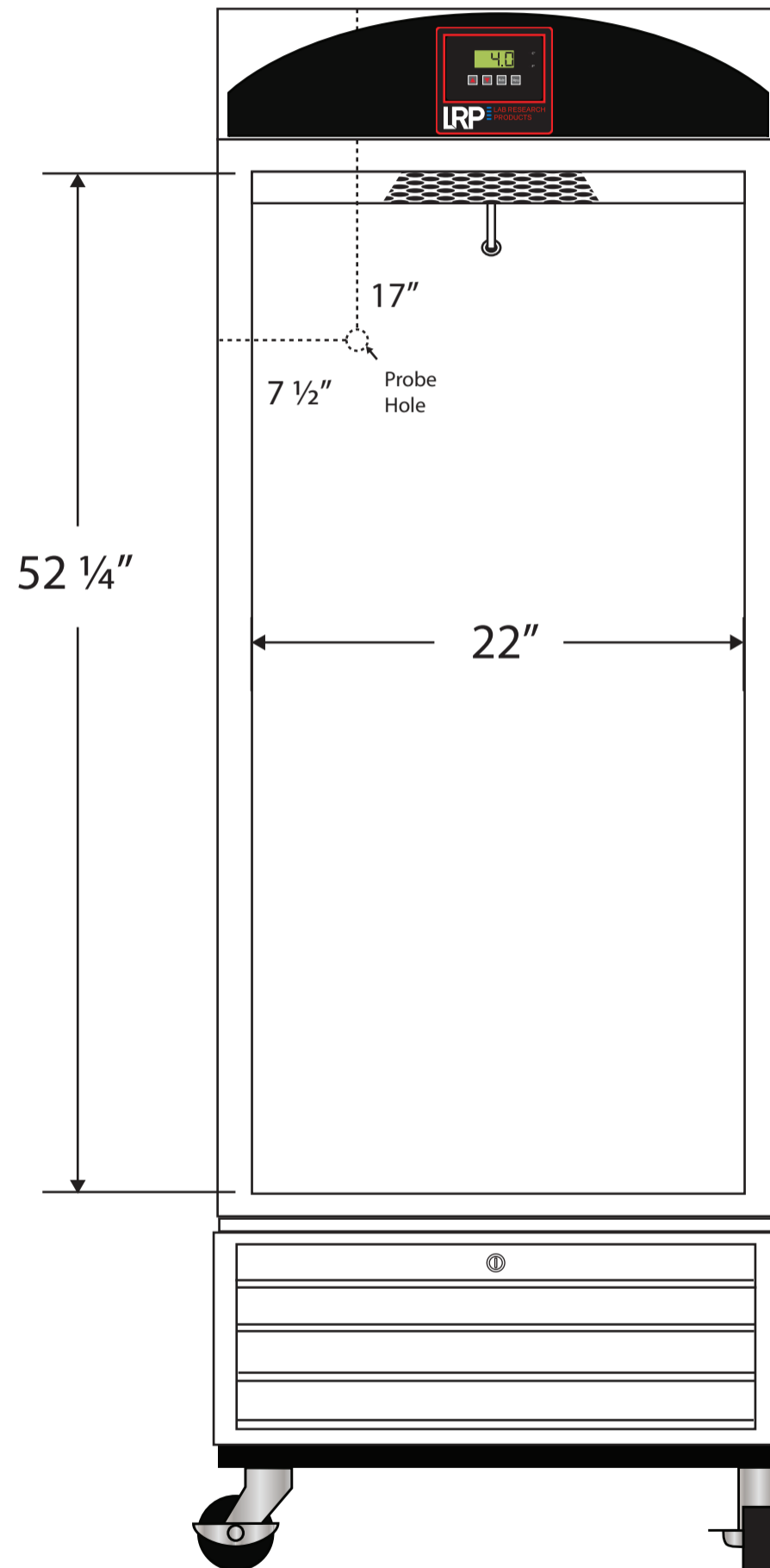
Front View
