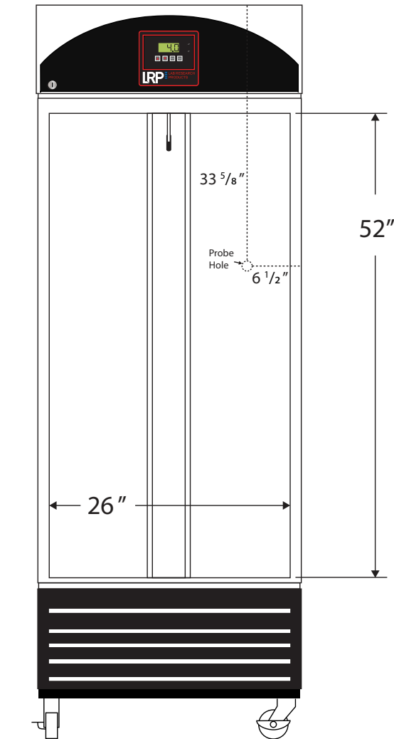
Front View
