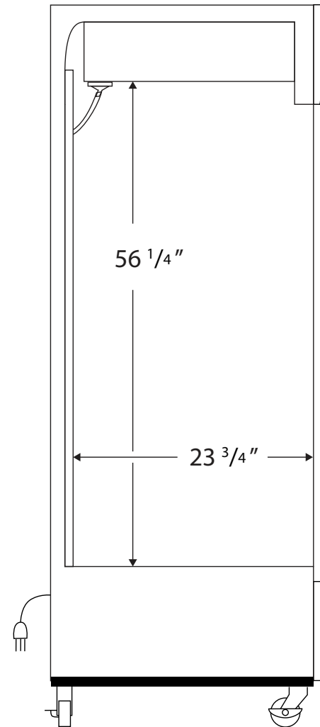
Side View
