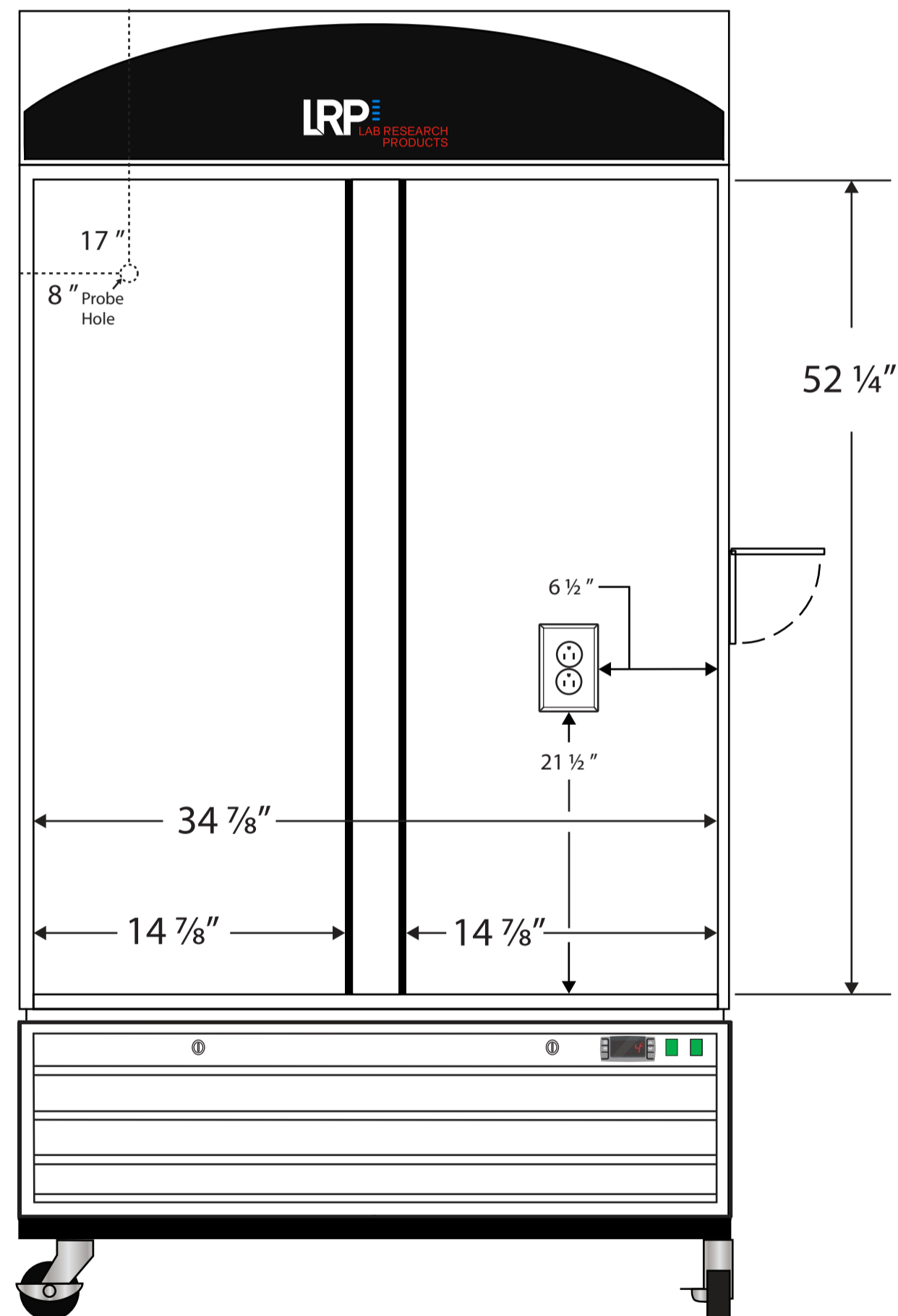
Front View
