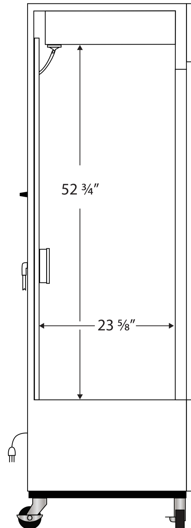
Side View
