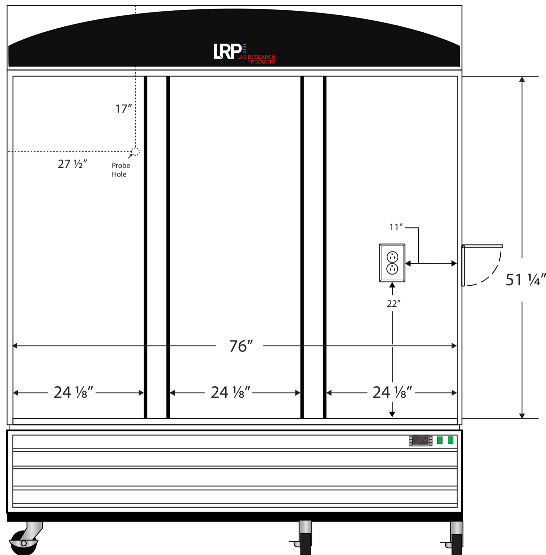
Front View
