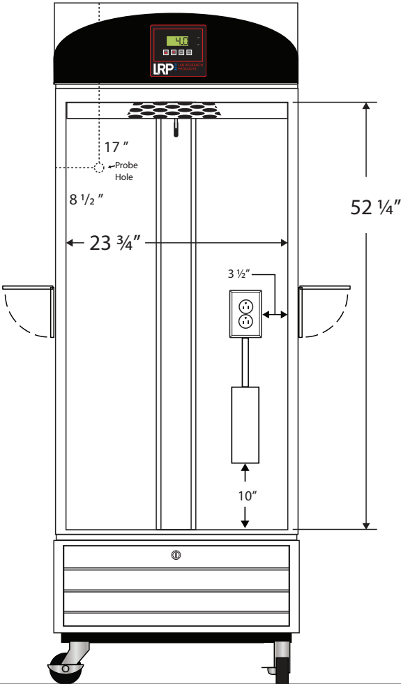
Front View
