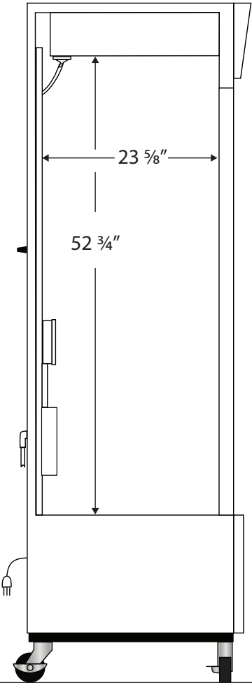
Side View
