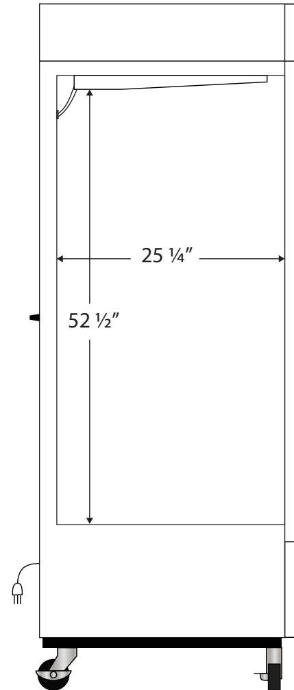
Side View
