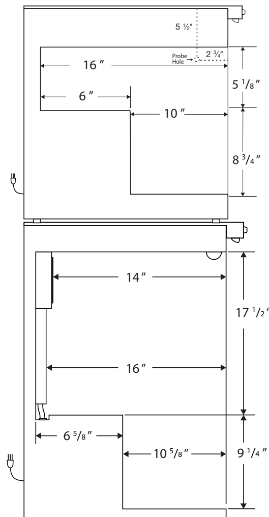
Side View
