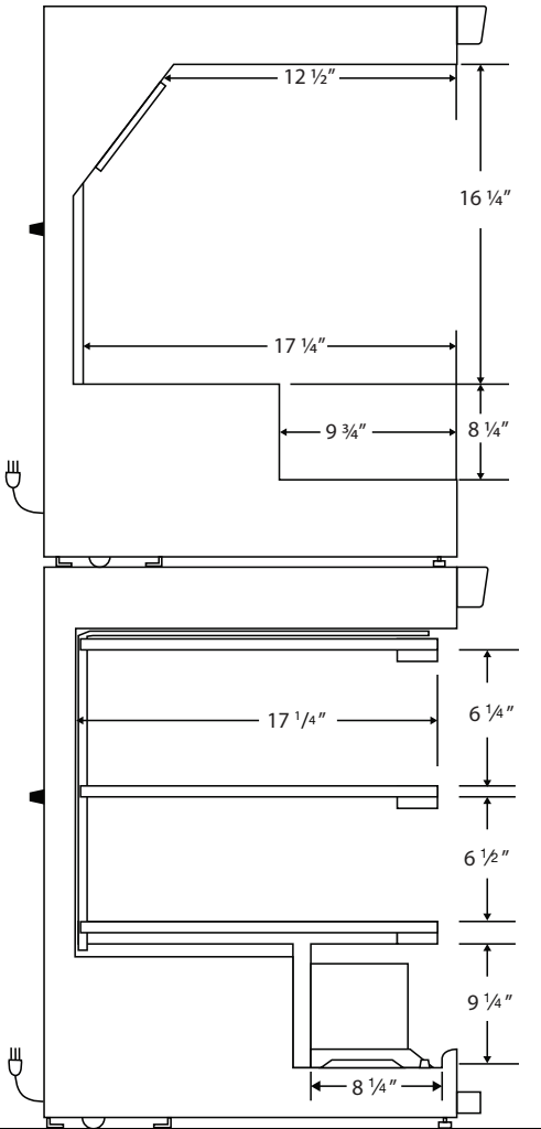
Side View
