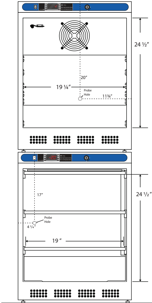
Front View
