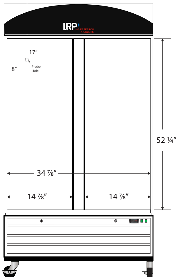
Front View
