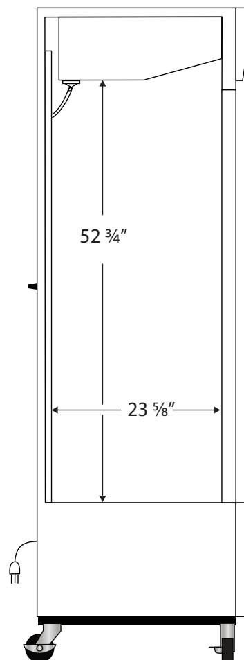
Side View
