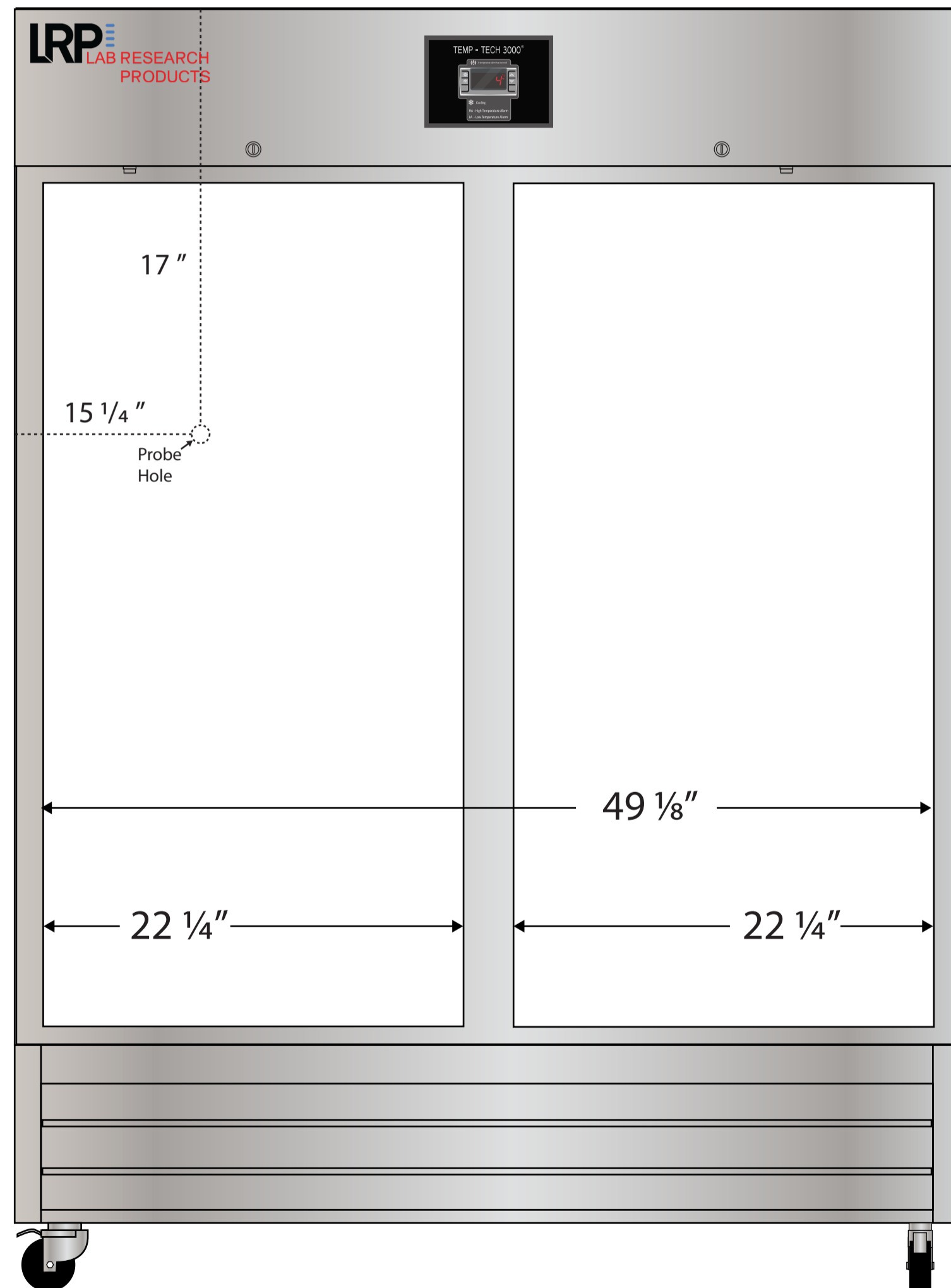
Front View
