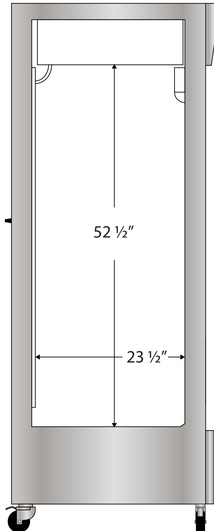
Side View
