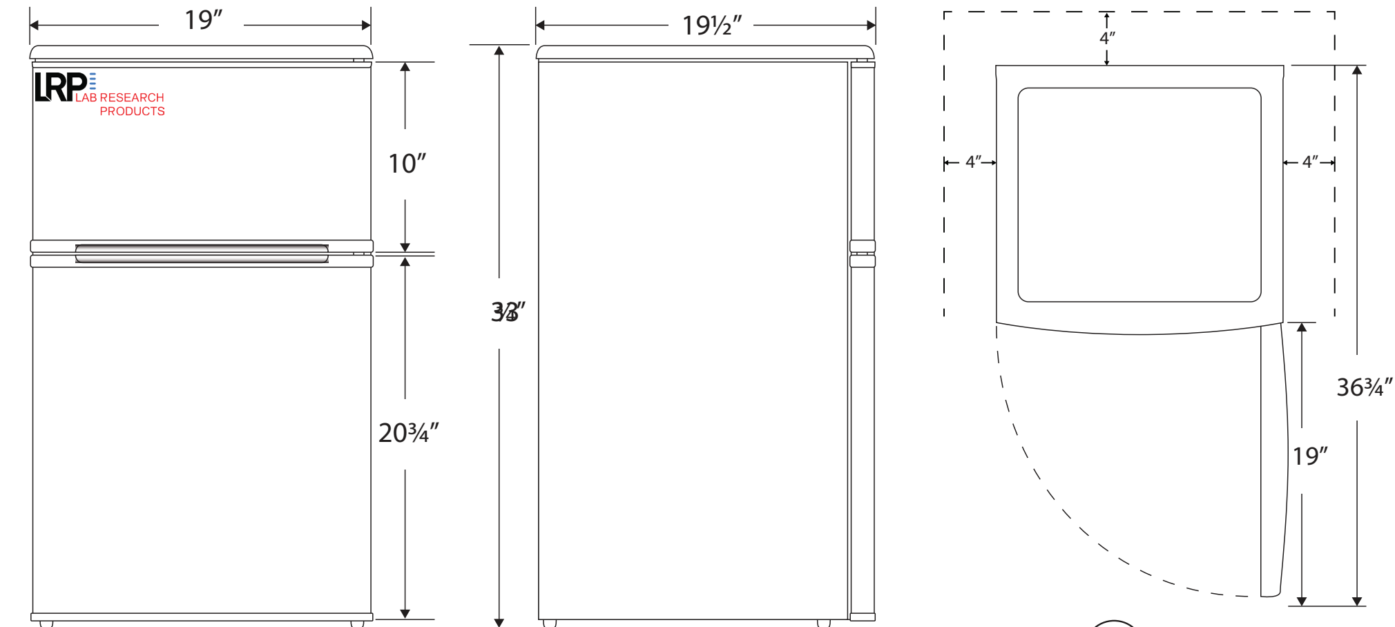
Top View
