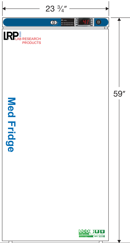
Front View
