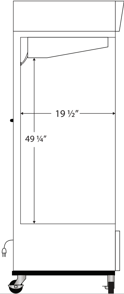
Side View
