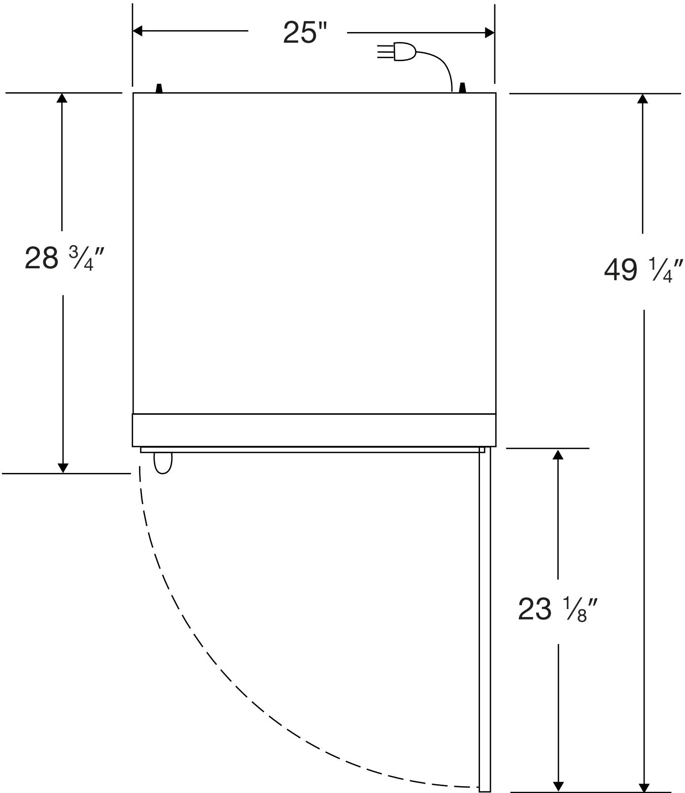
Top View
