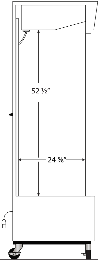
Side View
