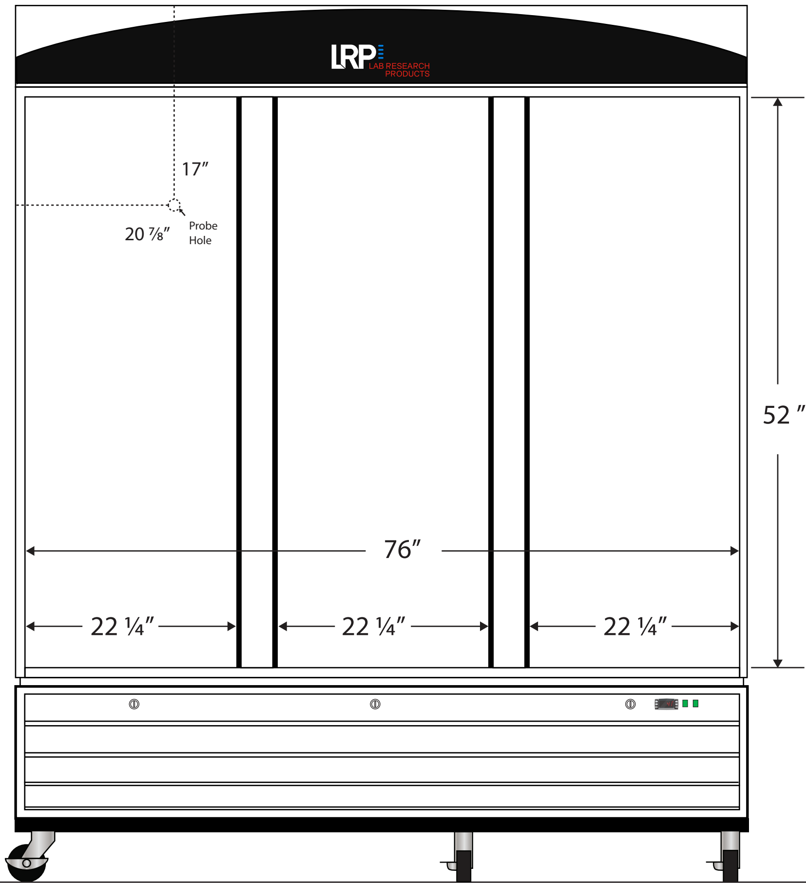
Front View
