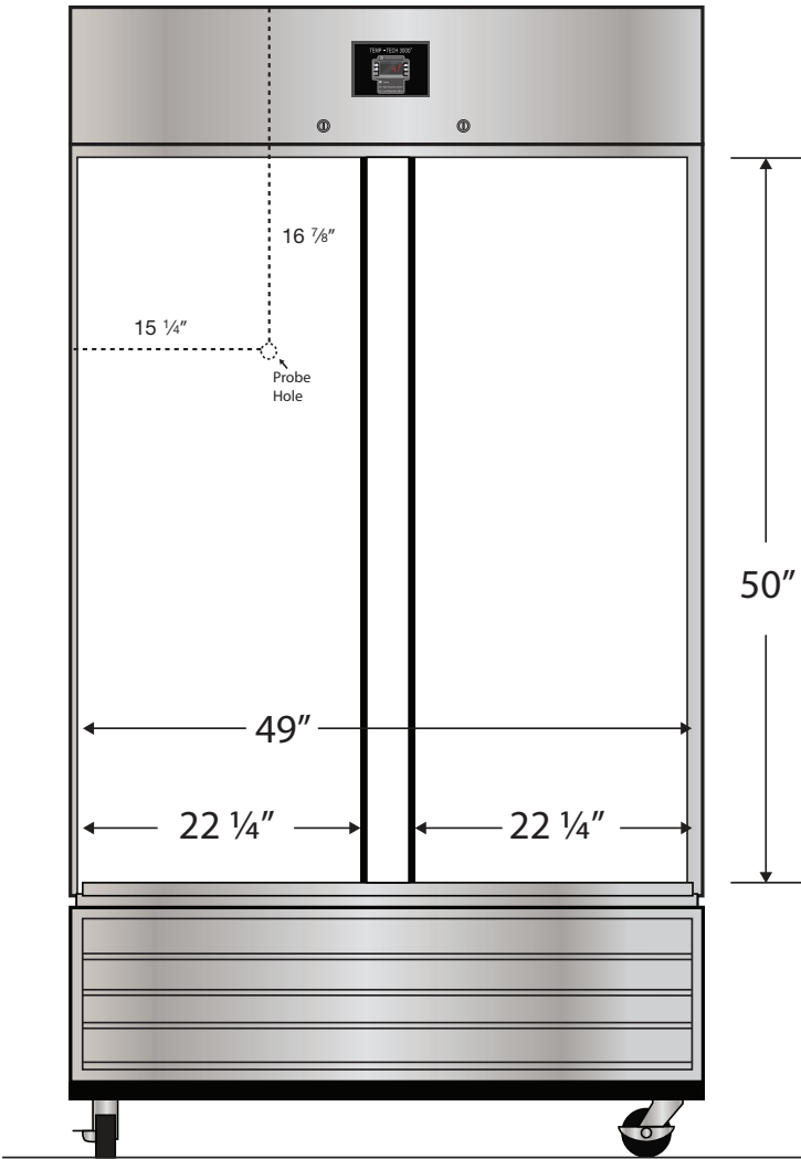
Front View
